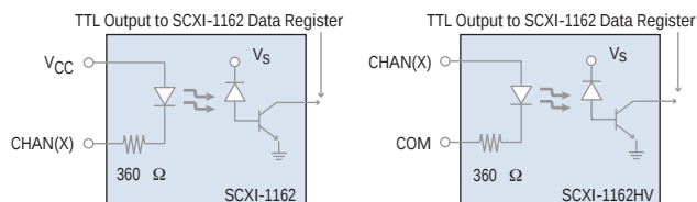
Figure 3. Digital Input Diagrams of the SCXI-1162 and the SCXI-1162HV
